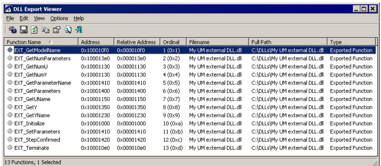
Figure 5.12. List of exporting functions by DLL Export Viewer utility
