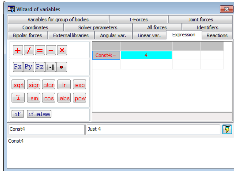
Figure 5.15. Constant-variable
